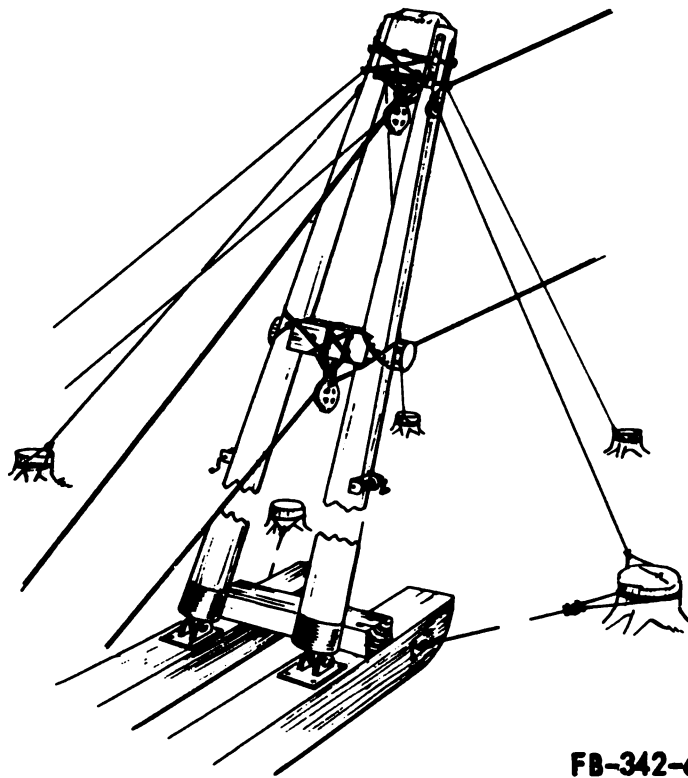
Figure 7-14. A-frame rigging and guying.
